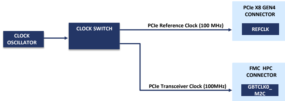
Figure 10: Clock for Root Port Application
